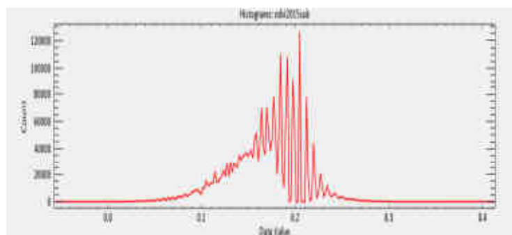
Figure 6: Histograms from NDVI for the 2015
