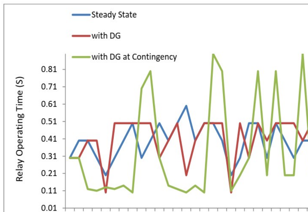
Figure 5: Relay Operating Time of 33-Bus Ilorin Feeder with DG at contingency
