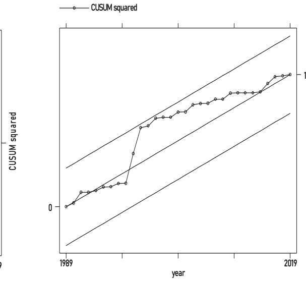
Figure 6b: CUSUM SQUARE
