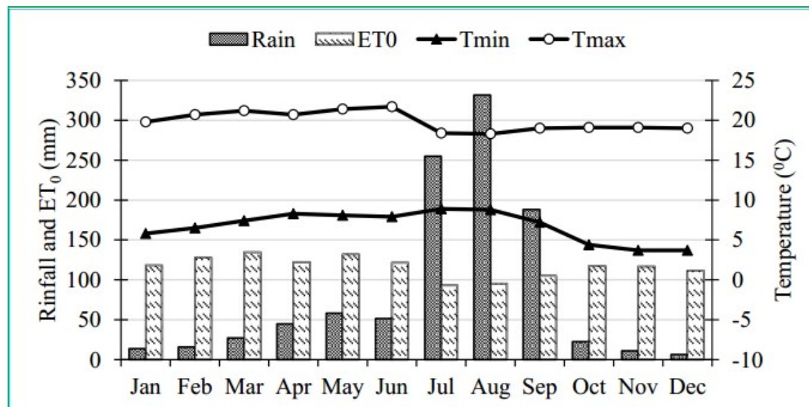
Figure 2. Average monthly rainfall, potential evapotranspiration (ET 0 ), maximum (T max ) and minimum (T min ) temperatures at Debre Berhan weather station (monthly data averaged from 2000 to 2014)
