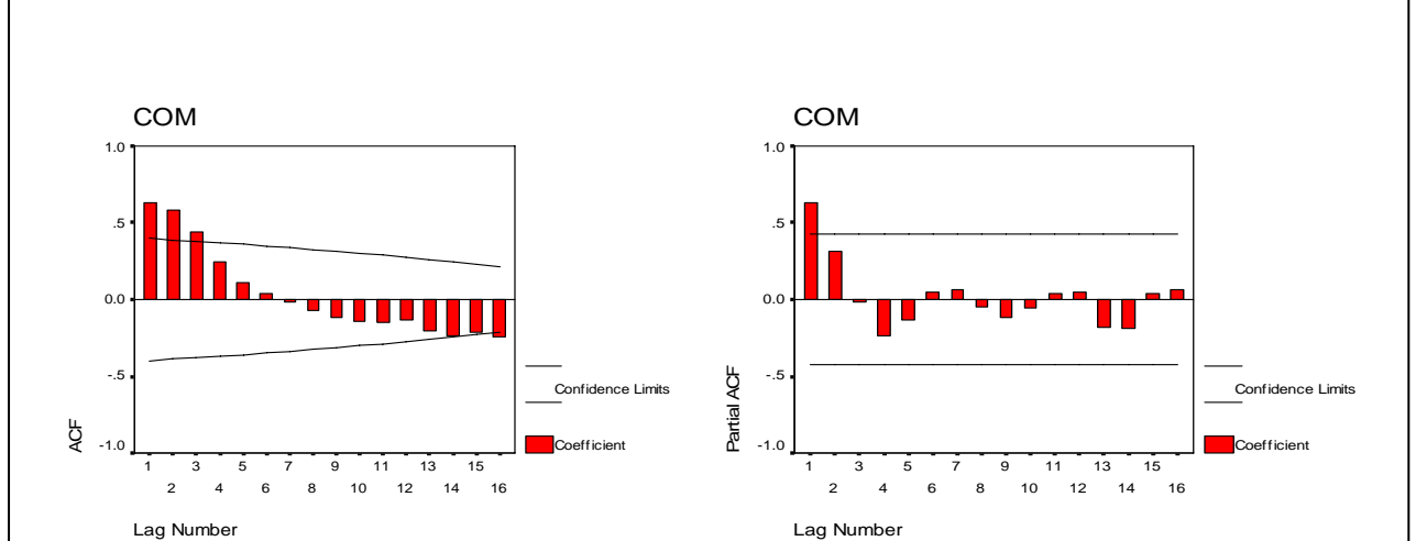
Figure 3: Autocorrelation and partial autocorrelation function of wholesale price at Jessore market
