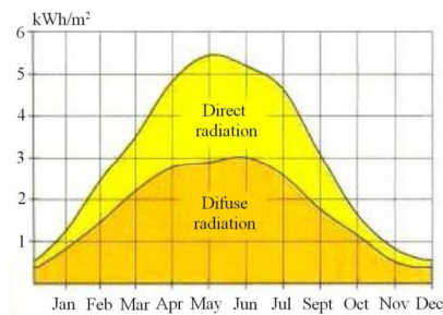
Fig. 1 Total and diffuse solar radiation
